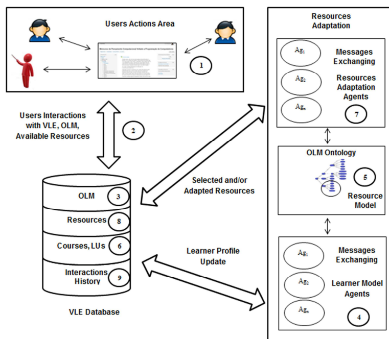
Figure 1. ArCARE Architecture [Bremgartner, Netto and Menezes 2017].
